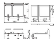
N-TZ-6060G
